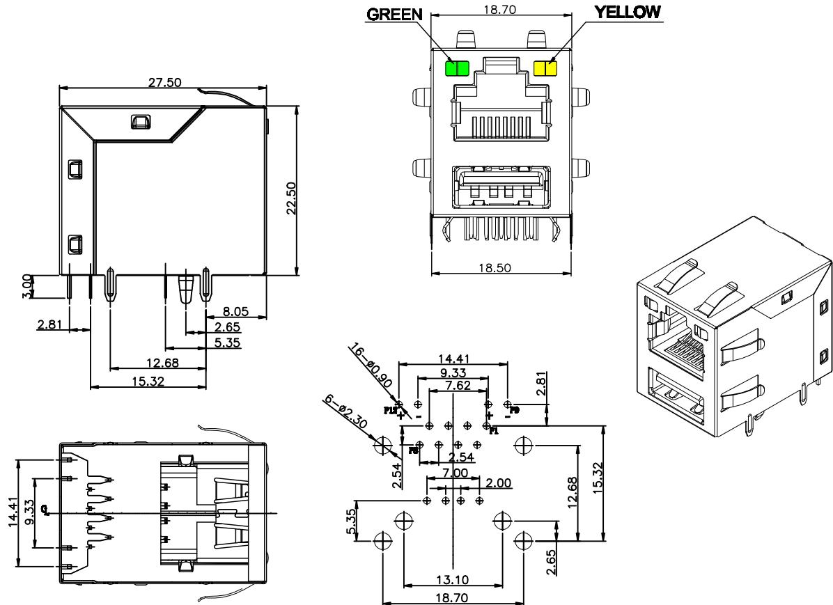
RECOMMENDED P.C.B LAYOUT TOP VIEW (COMPONENT SIDE)
